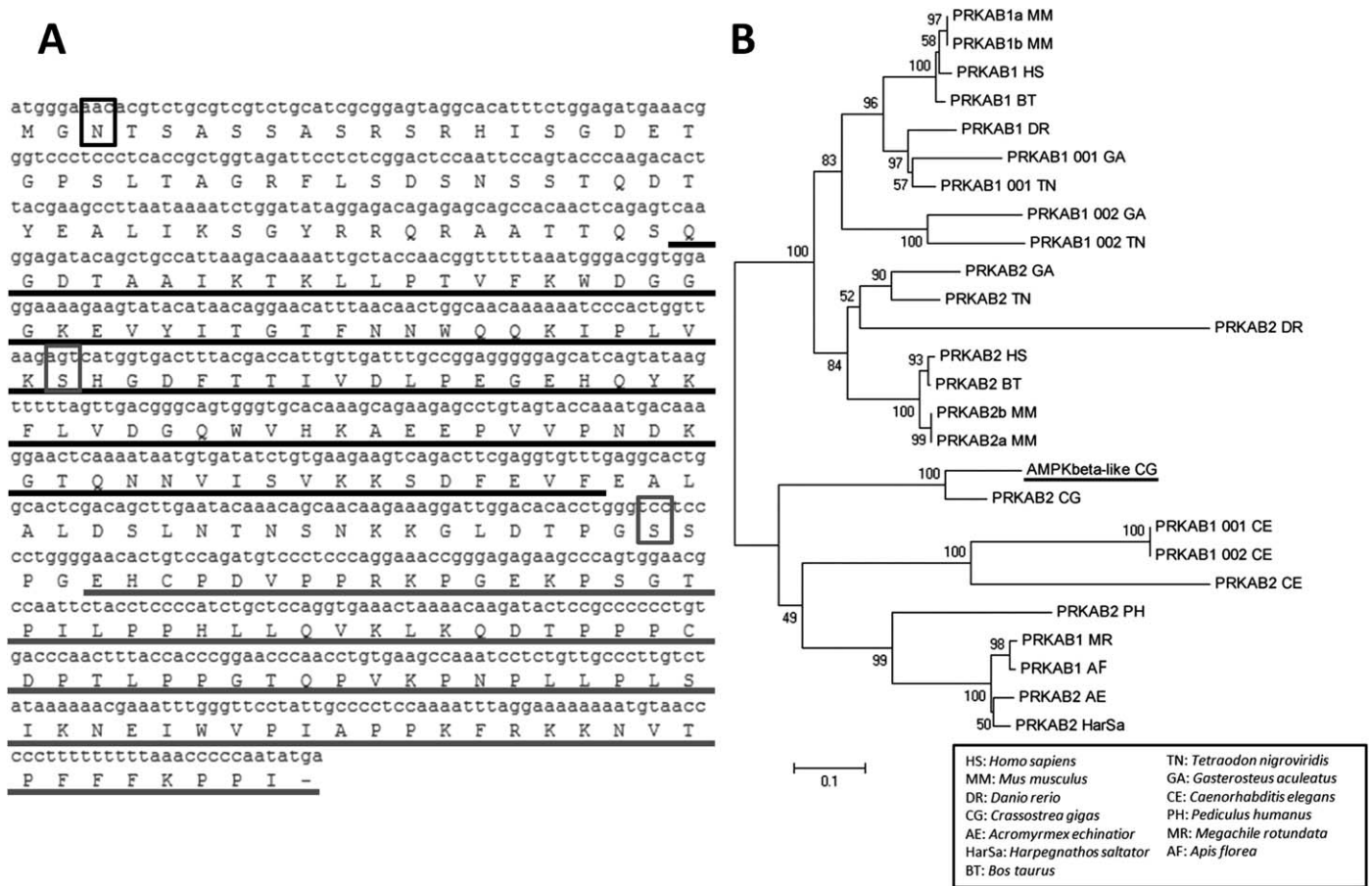
FIG. 1. A) Nucleotide and deduced amino acid sequences of Crassostrea gigas AMPK beta ( C. gigas _AMPK beta-like), obtained by merging three contigs matching AMPK beta2 (Sigenae accession numbers CU991642, FU6OSJA01AUVKV, and FU6OSJA01BDGCM). Black square, myristoylation site; gray squares, serine 108 and serine 182 phosphorylation sites; black underscore, beta-GBD. gray underscore, alpha gamma-SBS. B) Phylogenetic tree of AMPK beta compared to other AMPK beta subunits found in other species.
